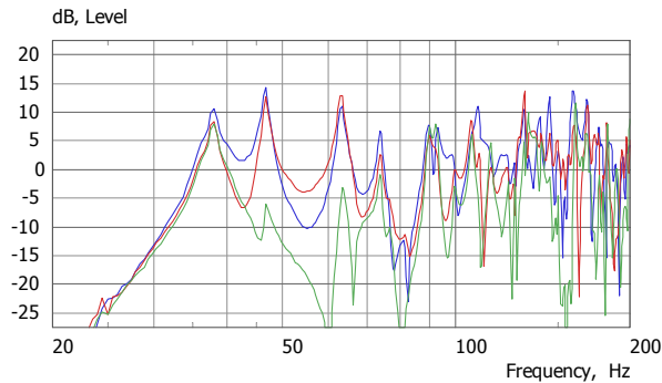
Fig. 5 Transfer function measured in reverberation chamber for 1x monopole , 1x cardioid , and 4x cardioids .
