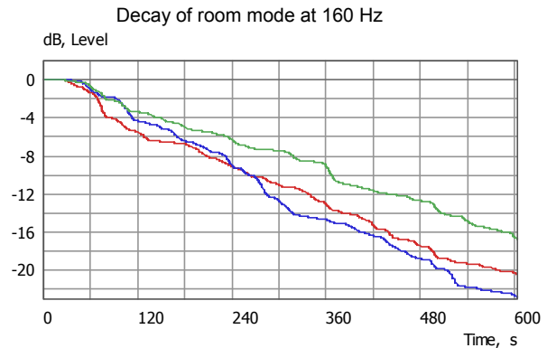
Fig. 4 Schroeder curves calculated for measurements taken in the reverberation chamber utilising 1x monopole , 1x cardioid , and 4x cardioids at 63Hz, 90Hz and 160Hz.
