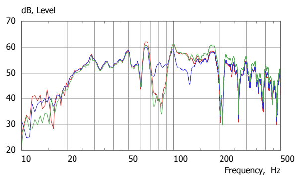
Fig. 8 Transfer function of summed centre channel and cardioid-array in listening room. Centre in-phase, centre 180° out-of-phase und wrong highpass filtering (uneven non-overlapping HPs)
