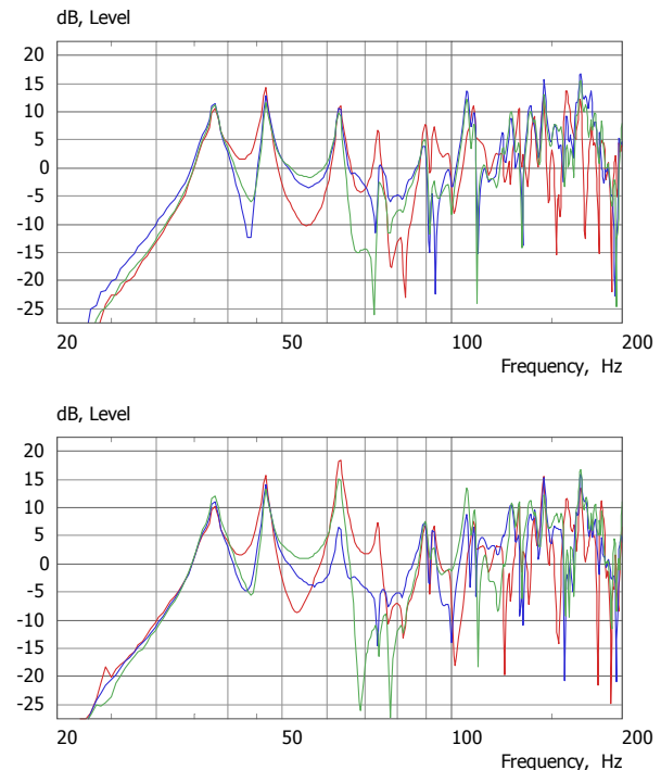
Fig. 6 Variation of modal excitation measured with four cardioid sources at 63Hz (110 Mode) and 74Hz (200 Mode). Changes were generated by varying the cardioid's orientation, their relative phase and level.
