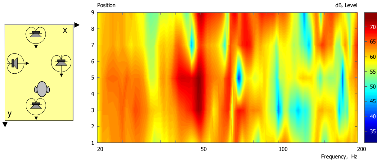
Fig. 11 Four cardioid subs: Contour plot of room transfer function plotted against measurement position (9 meas. positions, listening area ca. 1,5m 2 )
