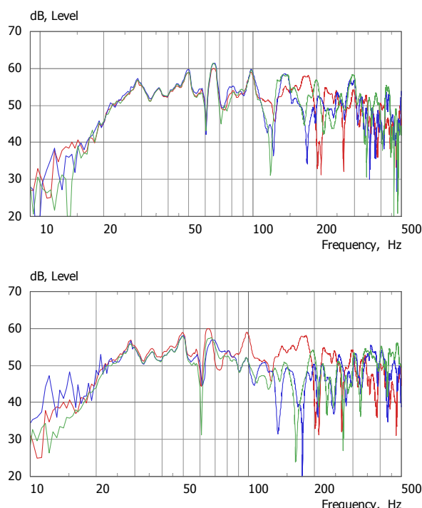
Fig. 7 5.1 multichannel sub-sat-configuration: transfer functions of individual channels summed with cardioid array (ca) in well damped listening room (decay times 20-200Hz 0,45-0,3s) top diagram: center front, left front and right front bottom diagram: center front, left rear and right rear
