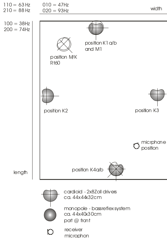
Fig. 2 Position, orientation, and number of cardioid subwoofers as used during the measurements.
