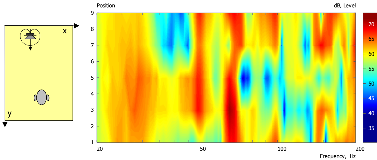
Fig. 9 One cardioid sub: Contour plot of room transfer function plotted against measurement position (9 meas. positions, listening area ca. 1,5m 2 )
